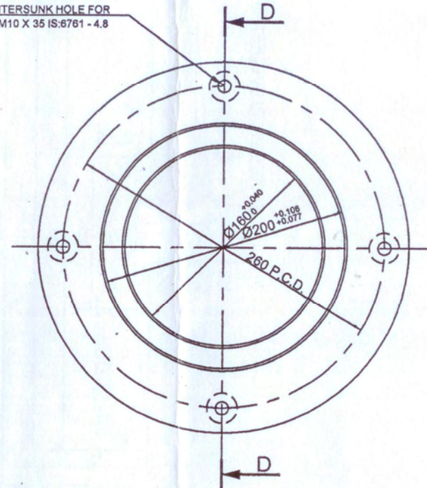
END VIEW
