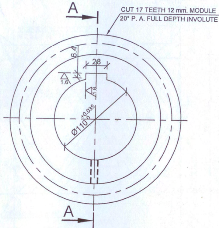
END VIEW
