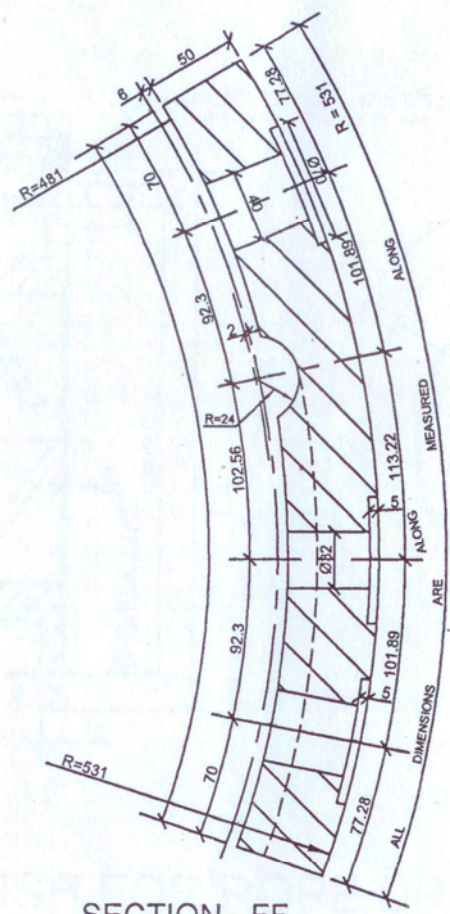
SECTION - FF
