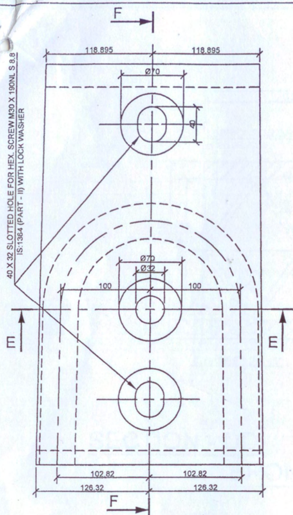
WIRE ROPE CLAMP MATERIAL :- C.S. GR. 340-570W OF IS:1030 PART NO.-07-17-02-00-02-02
