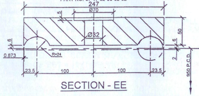
WIRE ROPE CLAMP MATERIAL :- C.S. GR. 340-570W OF IS:1030 PART NO.-07-17-02-00-02-02
