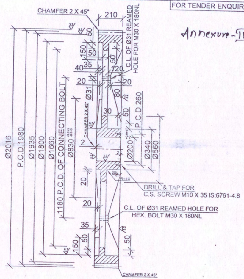
SECTION - AA
