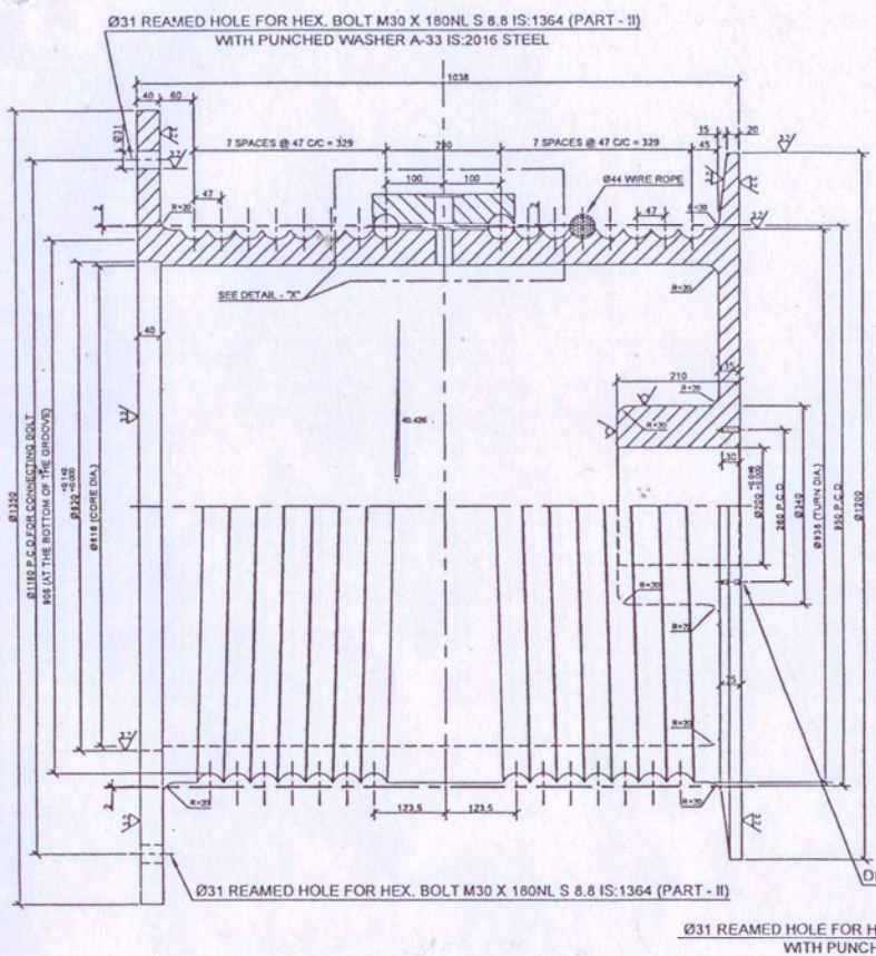
HALF SECTIONAL ELEVATION AT-AA D/S VIEW OF LEFT ROPE DRUM
